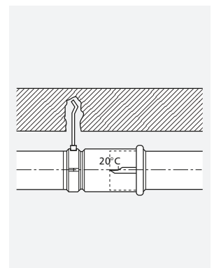
Horizontal assembly (e.g. at an ambient temperature of 20°C).
